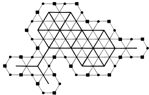
FIG. 8. An AB loop surrounding a cluster of bonds (heavy lines) on the superlattice. A and B spins on this loop are represented by heavy dots and squares, respectively. There is one large nonseparable cluster at the center, whose interior is divided into the twelve large triangles. Each of the four outside vertices is a nonseparable cluster consisting of just one SL site (they are the vertices with just one or three neighbors), and each of the four outside bonds (which connect these nonseparable clusters to each other and to the large nonseparable cluster) is a cutting link. The (perimeter) of the large nonseparable cluster has eight inward and two outward turns.
