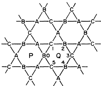
FIG. 1. The \sqrt{3} \times \sqrt{3} ground state of the kagomé lattice. The letters A , B , and C represent the spin directions illustrated in Fig. 2(b). The symbols P and Q and the labels 0–5 are the ones used in Appendix A.
