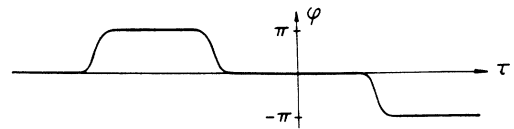
FIG. 6. An (+) instanton \overline{\varphi}^+(\tau) followed by two (-) instantons \overline{\varphi}^-(\tau) , where \tau is the (imaginary) time parameter.
