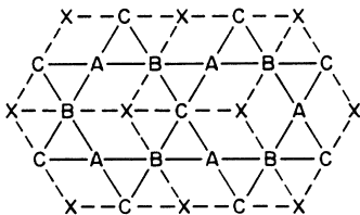
FIG. 7. The centers of kagomé hexagons (marked X ) form a triangular superlattice (SL). Connecting these by the dashed lines divides the plane into (large) rhombi, each with, say, an A -spin at its center, surrounded by four other sites.
