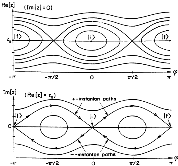
FIG. 5. Contours of constant \mathcal{H}(\varphi, z) . In (a), \text{Im}[z]=0 , and the contours in the (\varphi, \text{Re}[z]) plane depict ‘‘valleys’’ centered at (\varphi, z) = (0 \pmod{\pi}, z_g) . In (b), \text{Re}[z] = z_g , and the contours in the (\varphi, \text{Im}[z]) plane show ‘‘ridges’’ centered at (\varphi, z) = (\pm\pi/2 \pmod{\pi}, z_g) . The (+) instanton and (-) instanton tunneling paths are contours of \mathcal{H}=0 around these ridges.
