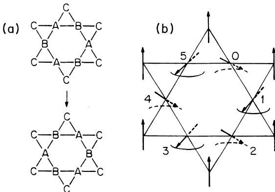
FIG. 3. The rigid-hexagon mode. All six spins on an ABABAB hexagon rotate collectively, as a rigid unit in spin space, by 180^\circ around the C direction, and end up forming a BABABA hexagon. The labels 0–5 correspond to the index l in Eqs. (2.4) and (2.5).
