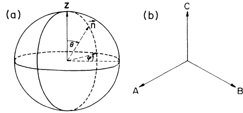
FIG. 2. (a) The unit vector \mathbf{n} = (\varphi, \theta) . (b) Types, A , B , and C spins on a triangle of the kagomé lattice. The common plane of A , B , and C , i.e., the “reference plane,” defines the \varphi = 0 and \pi directions in (a).
