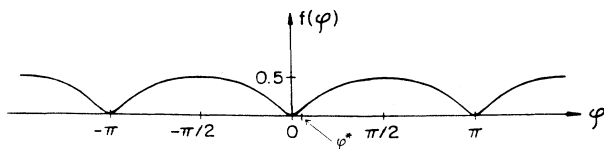
FIG. 4. A typical shape function f(\varphi) for the coplanarity potential \mathcal{H}_{\text{cop}} . The function shown here corresponds to the s=1 case of the function calculated in Appendix A, Eq. (A22), and used in Secs. IV C and V. The arrow shows the position of \varphi^* , which marks the crossover of f(\varphi) from quadratic to linear behavior. However, the general discussion of Secs. III and IV, up to Eq. (4.13), is independent of the particular shape of f(\varphi) , and only requires the symmetries of Eq. (2.6) to hold.
