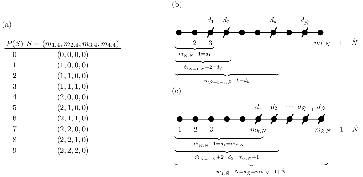
FIG. 4. Enumeration scheme of i-weights. (a) The first few i-weights of \mathfrak{su}(4) (excluding weights with m_{4,4} \neq 0 ), arranged in increasing order. (b) Illustration of the combinatorics underlying P_k(S) . (c) Striking out items such that each \tilde{m}_{\tilde{k}, \tilde{N}} takes on the largest possible value.
