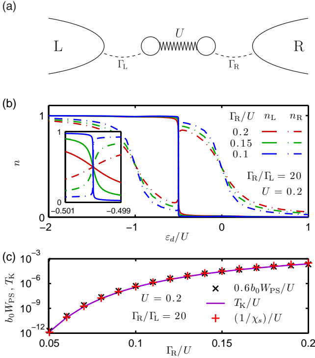
Figure 7: (Color online) (a) Cartoon of the Hamiltonian (47) for the asymmetric SIAM. (b) The occupations n_L (solid lines) and n_R (dashed lines) of the left and right level, respectively, as functions of \varepsilon_d , for several values of \Gamma_R , at a fixed ratio of \Gamma_R/\Gamma_L = 20 . As \varepsilon_d is lowered past the particle-hole symmetric point at \varepsilon_d = -U/2 , population switching occurs, with n_R changing from near 1 to near 0, and vice versa for n_L . Inset: zoom into the switching region around \varepsilon_d = -U/2 , showing that the switch is continuous (as function of \varepsilon_d ) even though the switching region becomes narrower for decreasing \Gamma_R . (c) Comparison of b_0 W_{PS} [from Eqs. (48) and (51), crosses], T_K [from Eq. (52), solid], and the inverse pseudospin susceptibility 1/\chi_s (pluses). All three quantities evidently decrease similarly with decreasing \Gamma_R/U .
