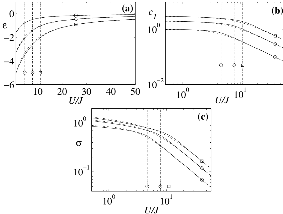
Fig. 3. (a) The ground state energy per site, \epsilon , (b) nearest neighbor correlation, c_1 = \langle a_{j+1}^\dagger a_j \rangle , and (c) variance of the number of atoms per site, \sigma^2 = \langle (n_j - \bar{n})^2 \rangle . Plots (b) and (c) use a log-log scale. The results of the DMRG (solid line) are obtained on a system with 128 sites, a maximum occupation number of 9 bosons per site and a reduced space of states of about 200 states. The estimates from the variational theory are plotted using dashed lines. The vertical lines mark the location of the phase transition according to [10]. The mean occupation numbers are denoted with circles ( \bar{n} = 1 ), diamonds ( \bar{n} = 2 ) and boxes ( \bar{n} = 3 ).
