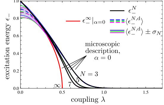
Figure S3: Lowest excitation energies of (dis-)ordered circuit QED systems with varying number of artificial atoms vs. coupling \lambda (in units of \omega = \Omega ). The figure shows the predictions the microscopic description if the \kappa -term is neglected ( \alpha = 0 ). The color code is the same as in Fig. S2. Furthermore, the analytical result for a homogeneous system with N \rightarrow \infty if the \kappa -term is neglected (red).
